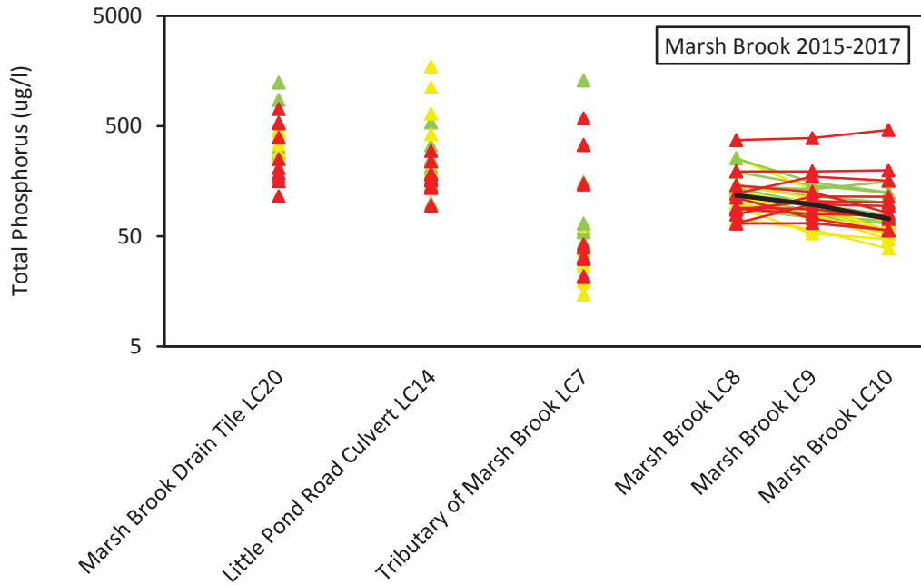
Figure 13. Total phosphorus “profile” along the main stem and tributaries of Marsh Brook from Marsh Brook Drain Tile (site LC20) downstream to the mouth of Marsh Brook (site LC10) during 2015-2017. The black line and triangles represent the median for each site, and the three colors represent data collected during 2015 (green), 2016 (yellow), and 2017 (red). Note the logarithmic scale on the y-axis.
